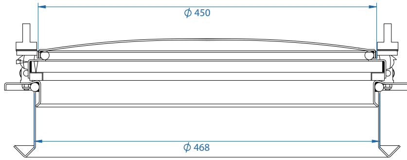
SECTION E-E
